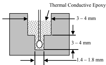
Figure 5. Section View of the 2 Stage Hole
