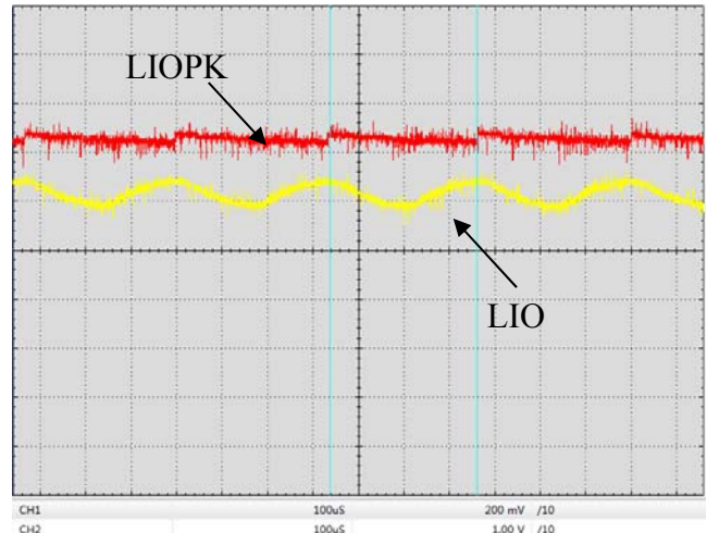
Figure 18. Digital Modulation Response at LIOPK & LIO Pin (f=3kHz)
