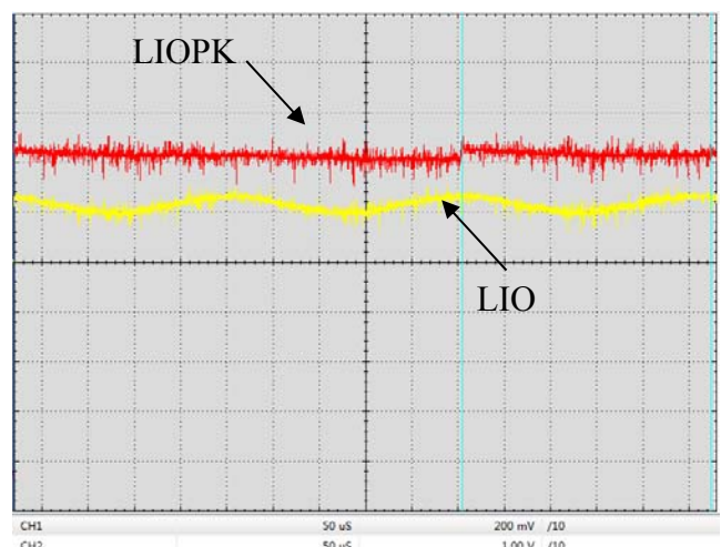
Figure 20. Digital Modulation Response at LIOPK & LIO Pin (f=4kHz)
